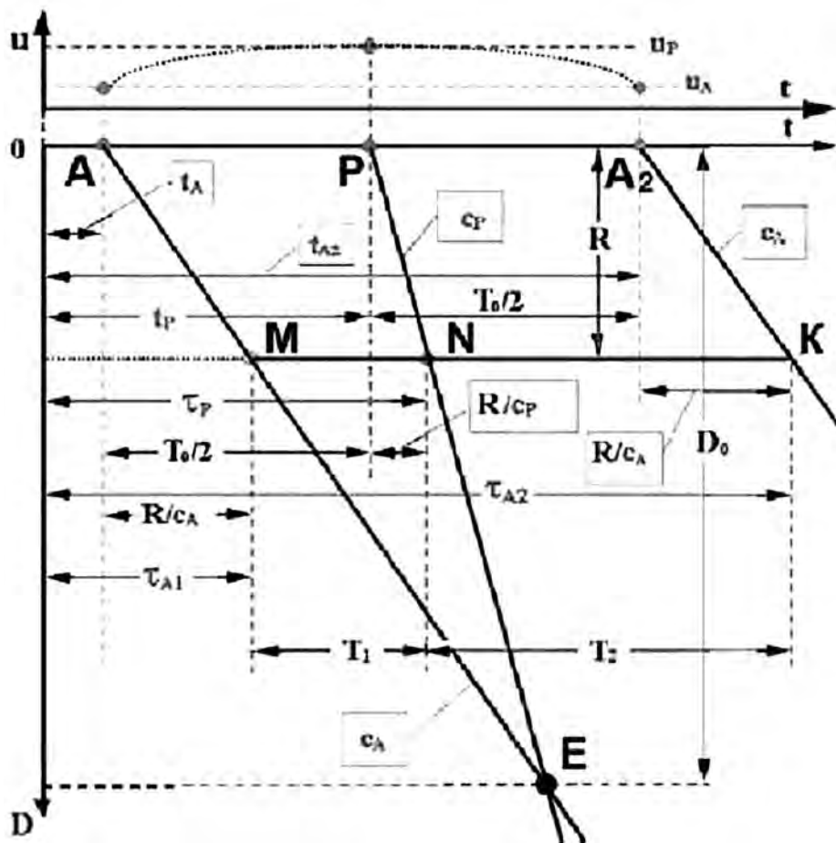
Fig. 2. Propagation of light in cosmos through large distances from sources moving at variable speeds ( T_0 = T_1 + T_2 ).
