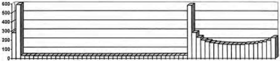
Fig. 6. Bursts of binary stars system brightness obtained by means of simulation for R \approx 1.8 D_0 (similar to novae or supernovae)
