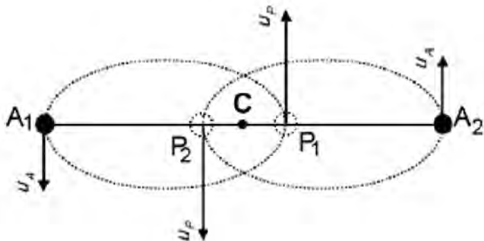
Fig. 1, Trajectories of two identical stars in a binary system orbiting along ellipses around a common centre of masses (C) coincident with common foci of two ellipses.
