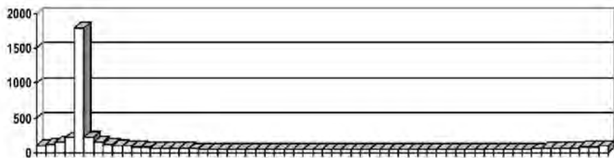
Fig. 3. A burst of binary star system brightness obtained by means of simulation for R \approx 0.7 D_0 (similar to novae or supernovae).
