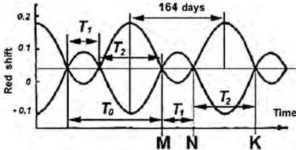
Fig. 7. Dependence in time of frequency spectrums of light from the object SS 433 as spectrums of a binary star system with an orbiting period equal to T_0 = 164 days (letters M, N and K denote the same events that are shown in fig.2).
