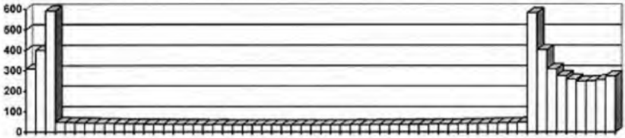
Fig. 5. Bursts of binary stars system brightness obtained by means of simulation for R \approx 1.2 D_0 (similar to novae or supernovae)
